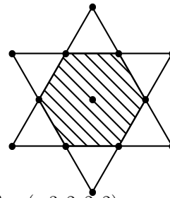
Figure 6: Monomials in multidegree \theta = (-3, 2, 2, 2)
