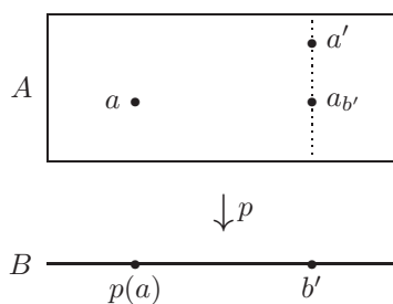
Figure 4: Metric fibration
