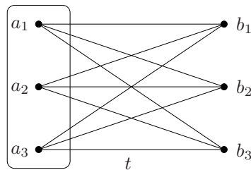
Figure 2: tK_{n,n} and its subspace 2tK_n , shown for n = 3 .
