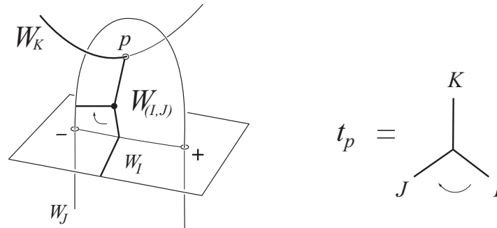
Figure 4: A local picture of the tree t_p = \langle (I, J), K \rangle associated to p \in W_{(I,J)} \cap W_K near a trivalent vertex adjacent to the edge of t_p passing through an unpaired intersection point p in a Whitney tower \mathcal{W} . On the left t_p is pictured as a subset of \mathcal{W} , and on the right as an abstract labeled vertex-oriented tree. In a non-simply connected 4-manifold X the edges of t_p would also be oriented and labeled by elements of \pi_1 X (as in Figure 5 below).
