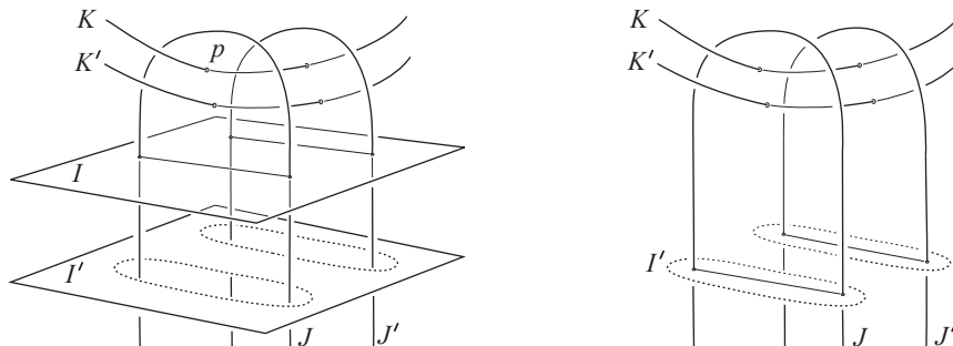
Figure 7: Extending a Whitney tower using parallel Whitney disks: An unpaired intersection point p \in W_{(I,J)} \cap W_K in a Whitney tower on A , where each of I, J and K contain exactly one occurrence of the index m , gives rise to eight unpaired intersections in four Whitney disks in the new Whitney tower on A' , formed from A by including a parallel copy of A_m . The dotted oval loops (left) bound neighborhoods of the Whitney arcs in the opaque I' sheet which have been perturbed into a nearby time coordinate along with the two corresponding translucent Whitney disks (right).
