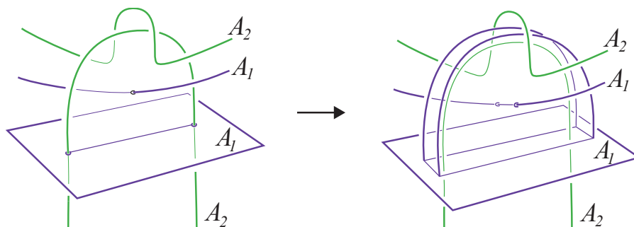
Figure 3: A Whitney move guided by the Whitney disk of Figure 2. The intersection between A_1 and the interior of the Whitney disk becomes a pair of self-intersections of A_1 after the Whitney move.
