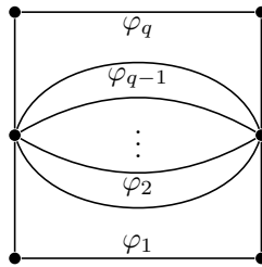
FIGURE 5. (\Gamma_0(xy) \setminus \mathcal{T})^0
