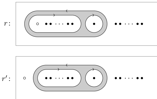
FIGURE 5.2. Pictures of maps r, r': P^n \rightarrow C_k(\mathbb{R}^n \setminus \{0\}) such that r_*([\partial P^n]) = \Delta_{j+1} - \Delta_j - \tau_1 and r'_*([\partial P^n]) = \tau_{j+1} - \tau_j - \tau_1 . In each case there are j + 1 fixed points in the bounded white region and k - j - 2 fixed points in the unbounded white region. The remaining point is in the shaded region; its position is parametrised by P^n .
