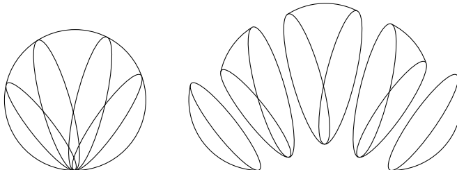
FIGURE 5.3. The slices of S^{n-1} when k = 5 .
