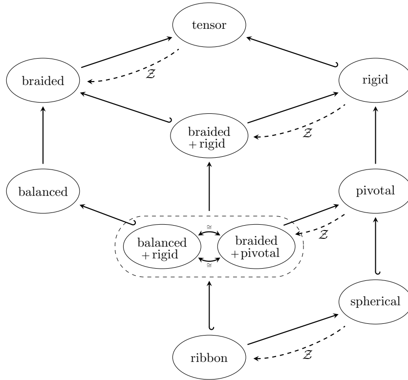
Figure 2: Synoptic chart of tensor categories
