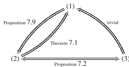
FIGURE 1. Paths in the proof of Theorem A
